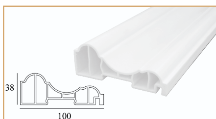
Nạp trang trí PWA 100-38 Pima Decorative Trim PWA 100-38 3000 x 100 x 38
