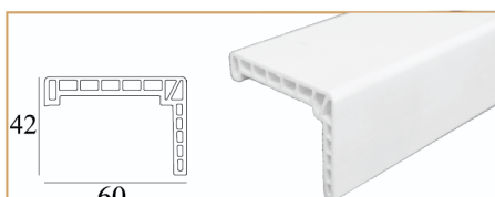
Phôi nẹp cửa Pima PWS-064 Pima Door Square Trim PWS-06022 1950-2300 x 60 x 42
