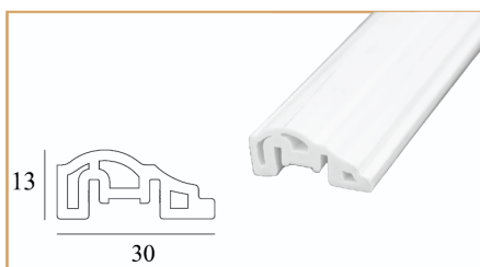
Nạp viền trang trí PWA 30-13 Pima Decorative Trim PWA 30-13 3000 x 30 x 13
