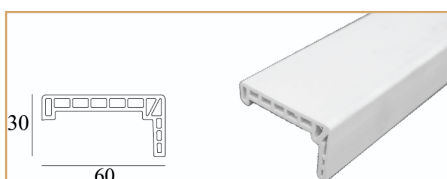
Phôi nẹp cửa Pima PWS-060 Pima Door Square Trim PWS-060 1950-2300 x 60 x 30
