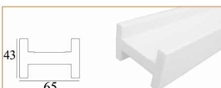
Thanh ray Pima PABT-6543 Pima RAILS PABT-6543 1950-2300 x 65 x 43
