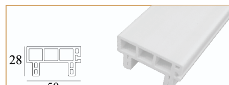
Phôi U đồ cửa Pima PWF-100H Pima Door Profile PWF-100H 1950-2300 x 50 x 28
