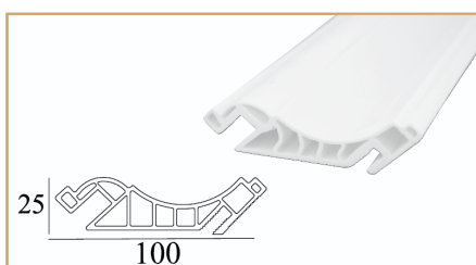
Nạp trần trang trí PWA 100-25 Pima Decorative Ceiling Trim PWA-10025 3000 x 100 x 25
