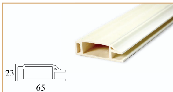
Thanh đồ cánh tủ PMK 6522 Cabinet Door Profile PMK 6522 3000 x 65 x 23
