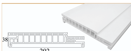
Phôi đồ cửa Pima PWF-200 Pima Door Profile PWF-200 1950-2300 x 202 x 38
