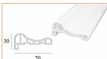
Nạp viền trang trí PWA 70-38 Pima Decorative Trim (With Cap) PWA-7038 3000 x 70 x 30
