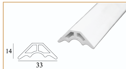
Nạp viền trang trí PVT 3314 Pima Decorative Trim (V INNER ANGLE) PVT 3314 3000 x 33 x 14
