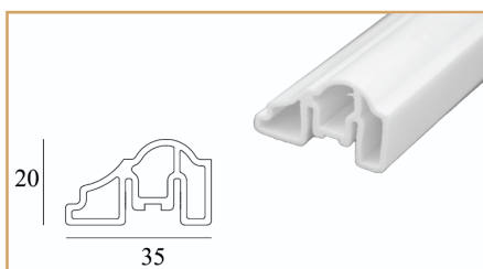
Nạp viền trang trí PWA 35-20 Pima Decorative Trim PWA 35-20 3000 x 35 x 20
