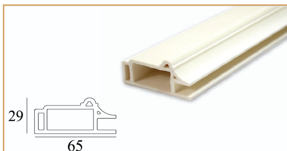
Thanh đồ cánh tủ PMK 6528 Cabinet Door Profile PMK 6528 3000 x 65 x 29
