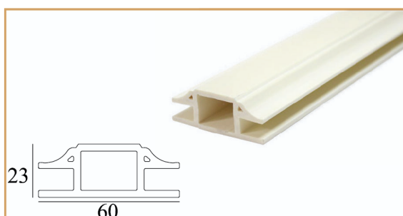
Đồ giữa cánh tủ PMK 6022 Central Cabinet Door Profile PMK 6022 3000 x 60 x 23
