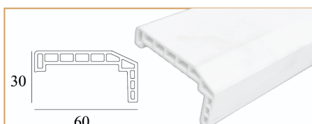
Phôi nẹp cửa Pima PWV-060 Pima Door Square Trim PWV-060 1950-2300 x 60 x 30
